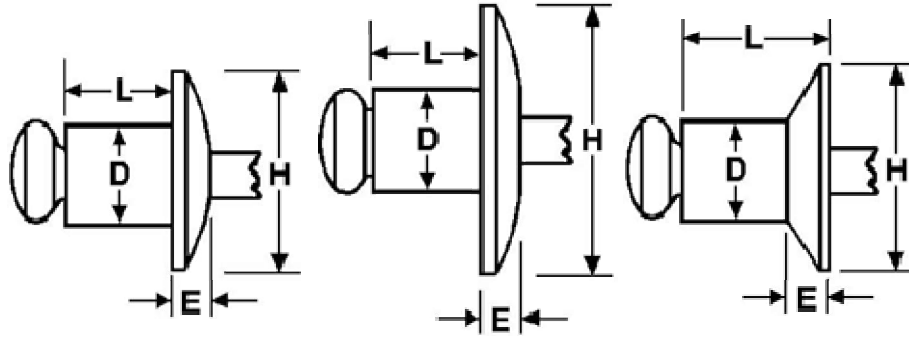
Button Head Large Flange Countersunk 5056 Aluminum Body - Coated Steel Mandrel - IFI Grade 19
