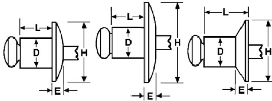
Button Head
