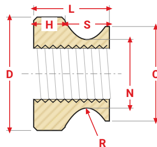
SECTION VIEW • 1/64" × 45° CHAMFERS
